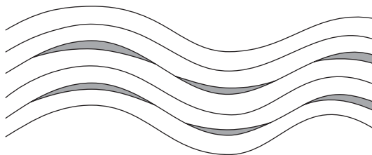
(b) Corndon Hill phacolith
