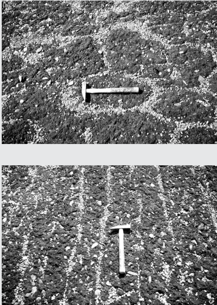
Plate 11.3 (a) Sorted polygons and (b) sorted stone stripes, Svartisen, northern Norway. The polygons and the stripes are found at the same site, the polygons on a very gently sloping area and the stripes on the steeper slope below. (Photographs by Wilfred H. Theakstone)
