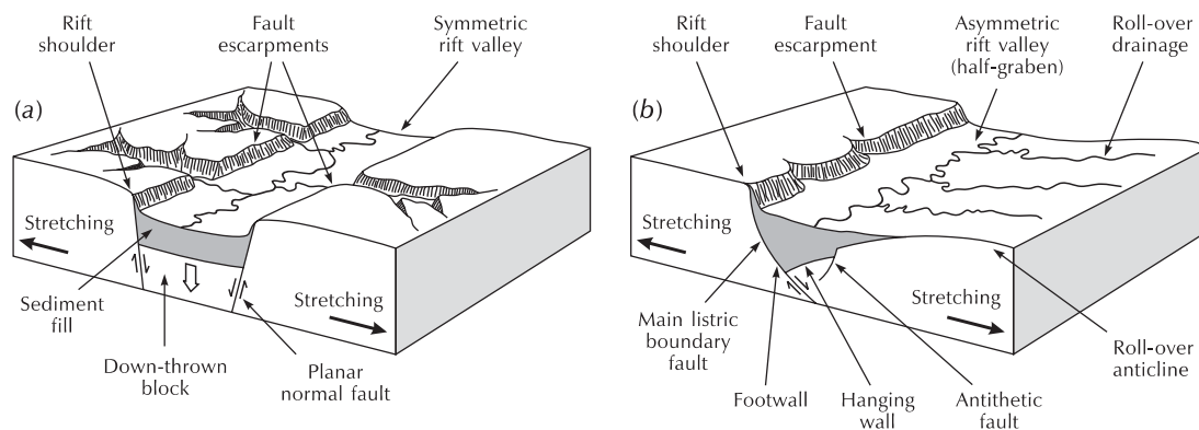
Figure 5.24 Down-faulted structures. (a) Graben. (b) Half-graben.
