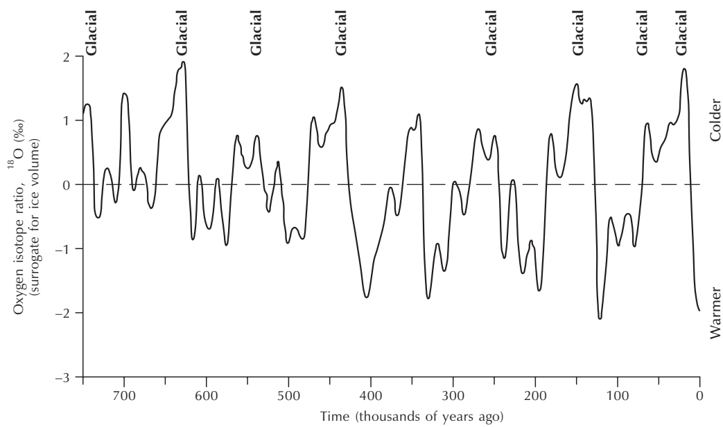
Figure 10.4 Temperature changes over the last 750,000 years, showing alternating colder (glacial) and warmer (interglacial) stages.
