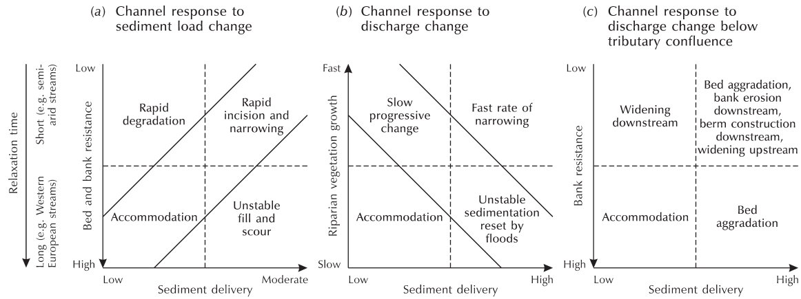
Figure 9.13 Domains of channel change in response to changing sediment load and discharge in different regions. Responses are to (a) a dominant reduction in sediment loads, (b) a dominant reduction in floods. (c) The special case of channel change below a tributary confluence in a regulated river dominated by flood reduction.
