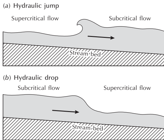
Figure 3.10 (a) Hydraulic jump. (b) Hydraulic drop.
