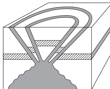
Figure 5.2 Minor intrusions. (a) Laccoliths and associated features (dykes, sills, and bysmaliths). (b) Cone sheets.
