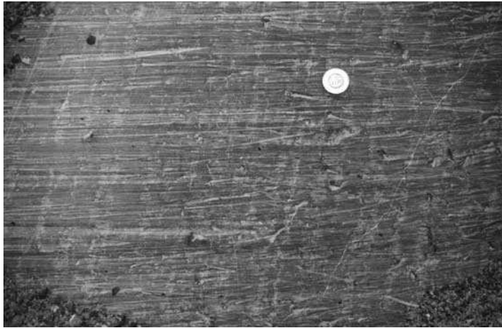
Plate 3.4 Striated limestone bedrock near the snout of Saskatchewan Glacier, Canadian Rockies. (Photograph by Mike Hambrey)
