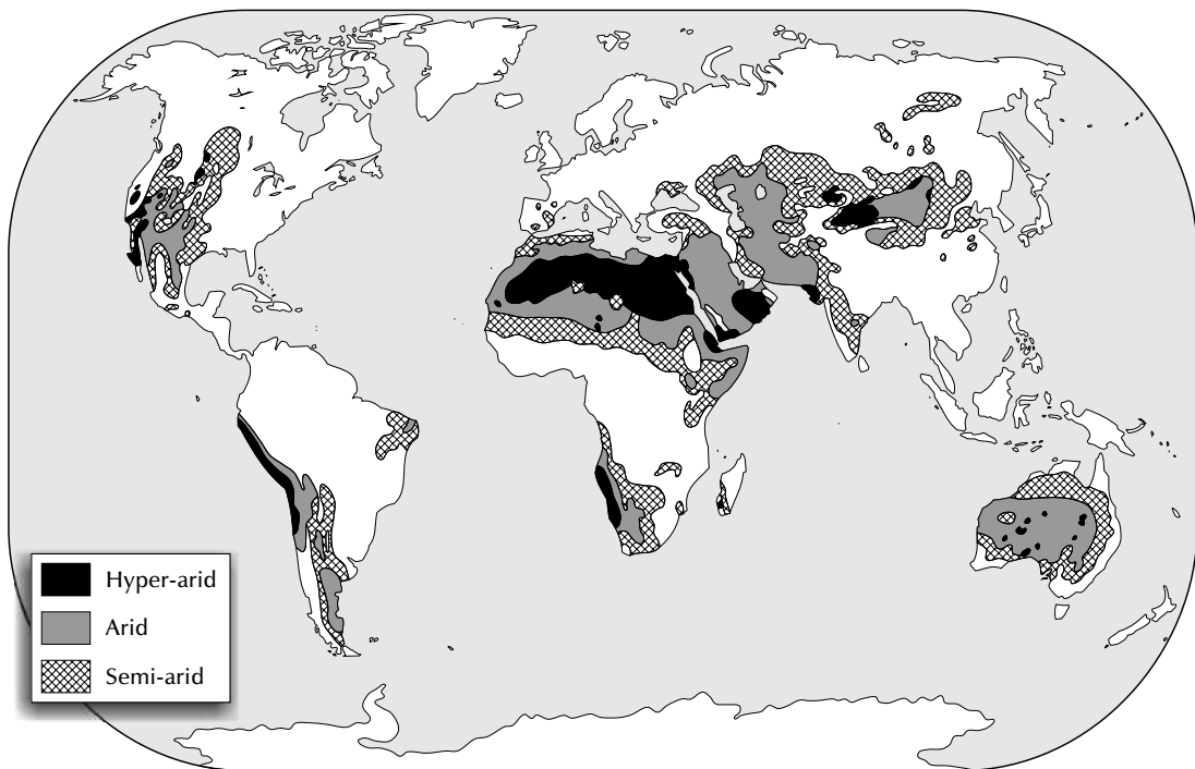
Figure 12.1 The world's deserts.
