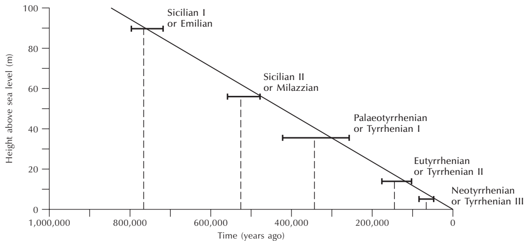
Figure 14.10 Quaternary sea-levels in the Mediterranean: the classic interpretation.
