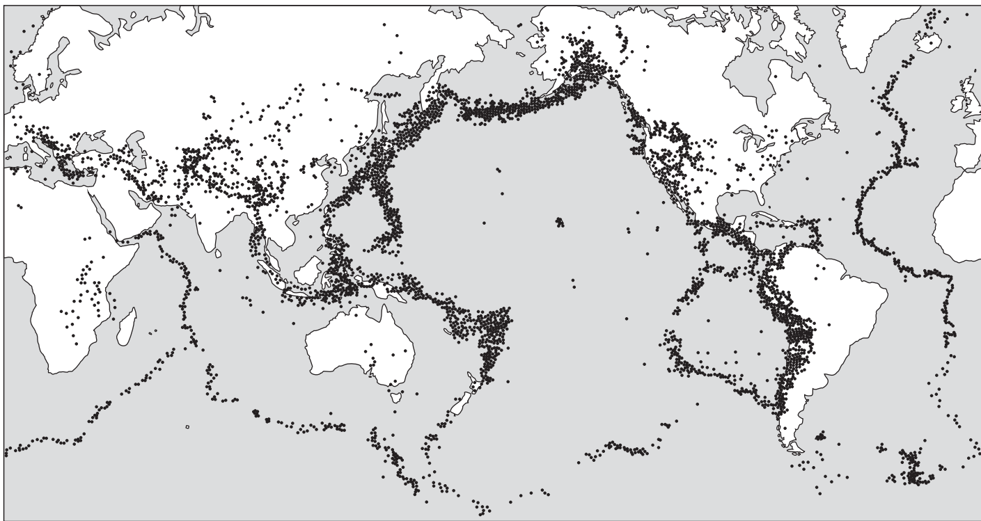
Figure 4.5 Global distribution of earthquakes. Source: Adapted from Ollier (1996)
