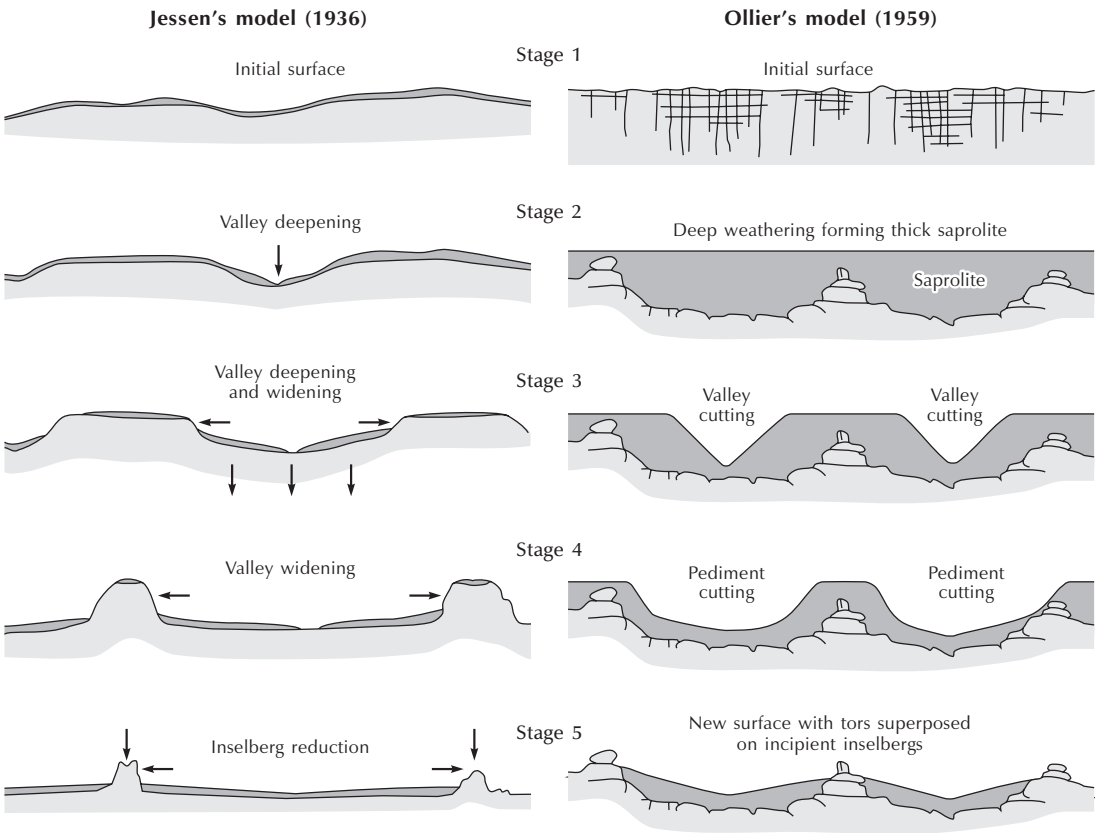
Figure 15.3 Theories of etchplanation. Source: Adapted from Jessen (1936) and Ollier (1995)
