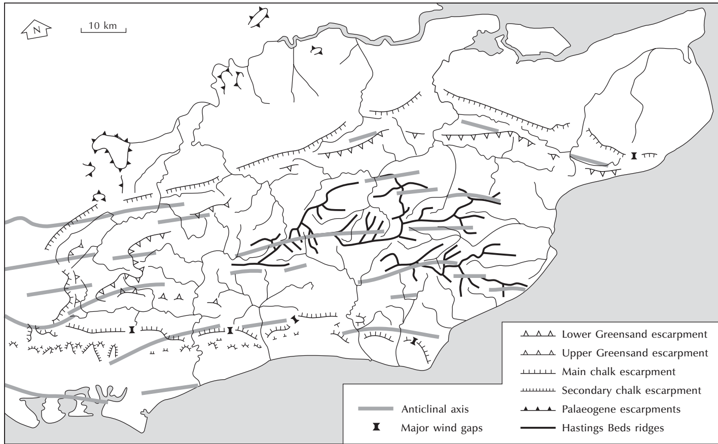
Figure 5.15 Some structurally influenced topographic features in south-east England.
