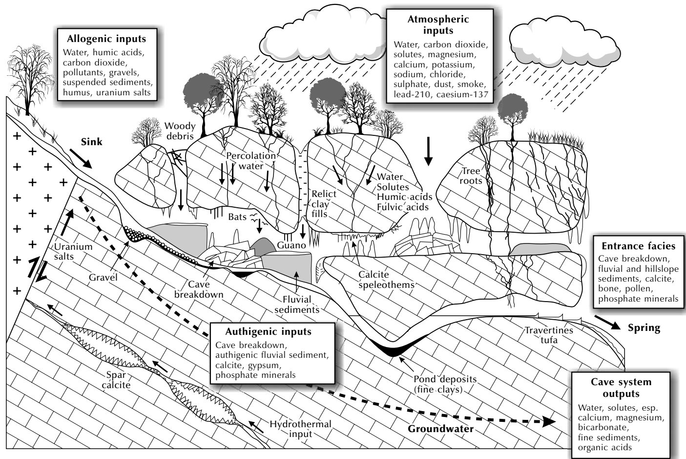
Figure 8.17 The cave system.
