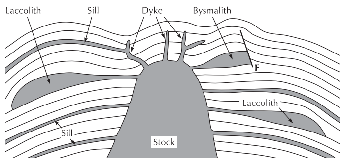
Figure 5.2 Minor intrusions. (a) Laccoliths and associated features (dykes, sills, and bysmaliths). (b) Cone sheets.
