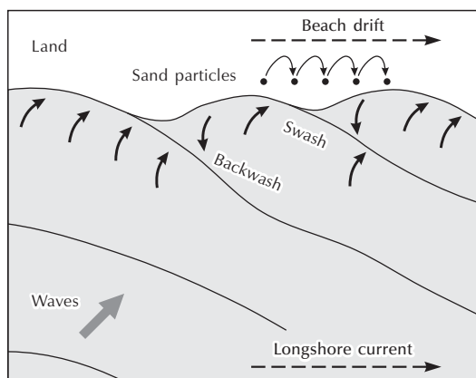
Figure 3.18 Beach drift.
