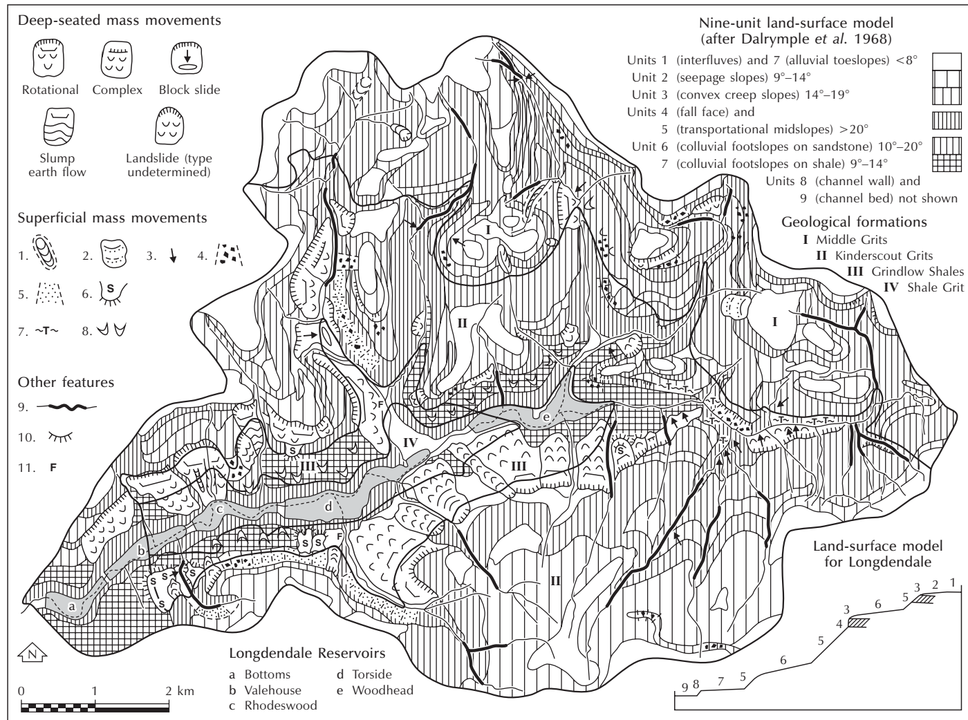
Figure 1.6 Morphological map of Longdendale, north Derbyshire, England. The map portrays units of a nine-unit land-surface model, types of mass movement, and geological formations. The superficial mass movements are: 1 mudflow, earthflow, or peat burst; 2 Soil slump; 3 Minor soil slump; 4 Rockfall; 5 Scree; 6 Solifluction lobe; 7 Terracettes; 8 Soil creep or block creep and soliflucted material. The other features are: 9 Incised stream; 10 Rock cliff; 11 Valley-floor alluvial fan.
