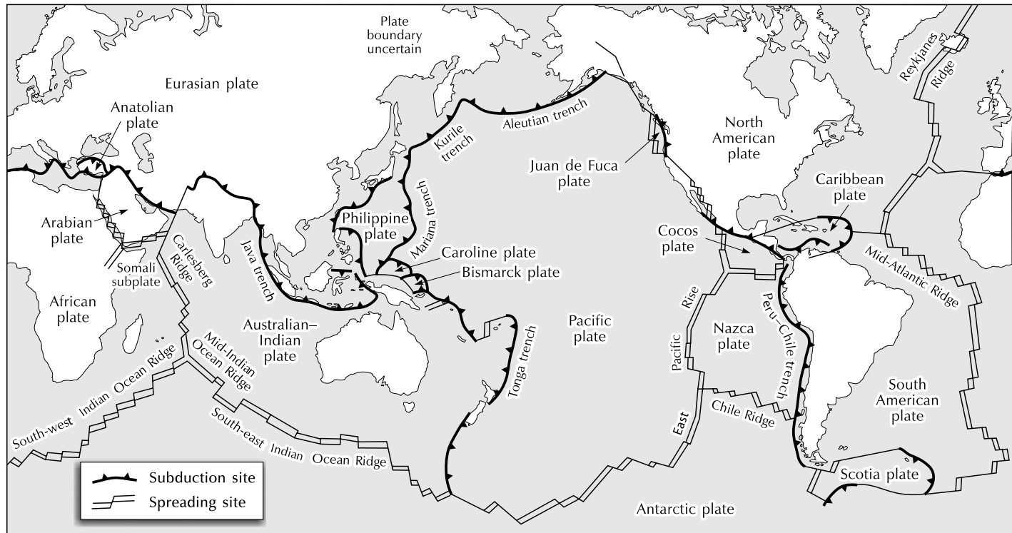
Figure 4.2 Tectonic plates, spreading sites, and subduction sites.
