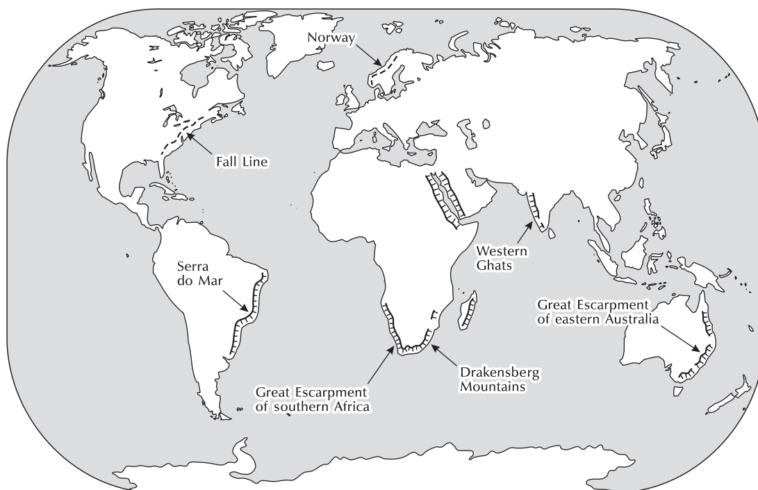
Figure 4.8 Great escarpments on passive margins.
