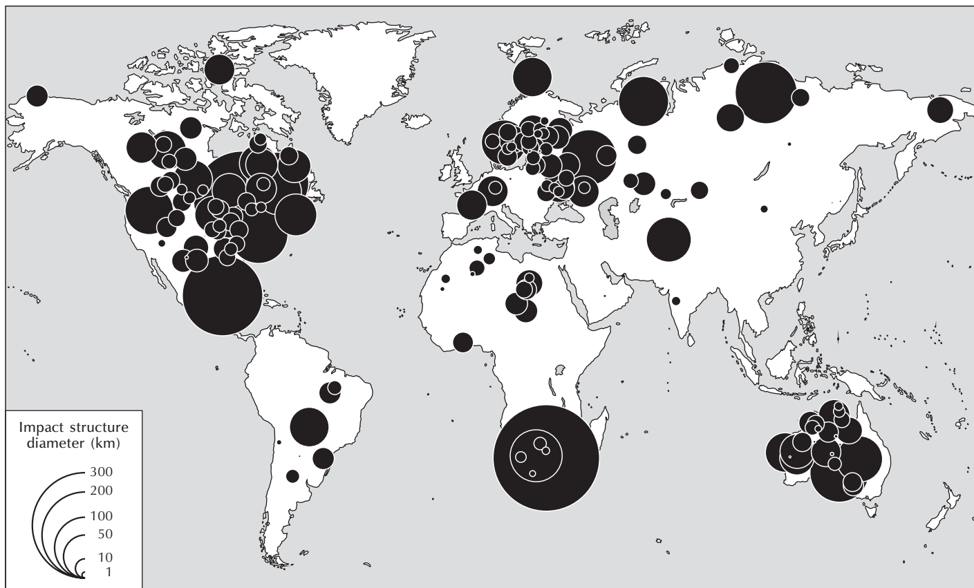
Figure 5.12 The distribution of known impact craters.
