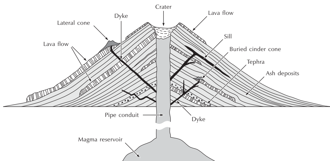
Figure 5.5 The structure of a typical strato-volcano.
