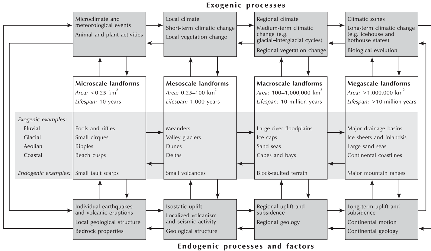
Figure 1.1 Landforms at different scales and their interactions with exogenic and endogenic processes.
